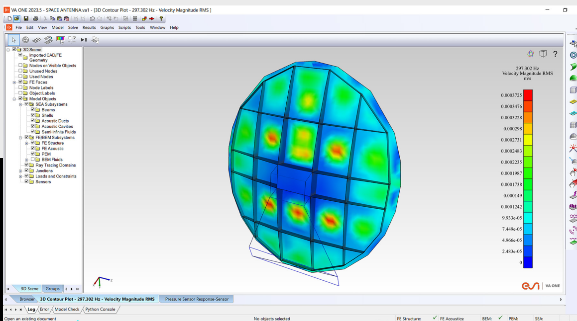
Analyzing the vibroacoustic response of an antenna subjected to diffuse acoustic field loading to optimize performance and ensure structural integrity. © ESI Group (a part of Keysight Technologies), 2025
