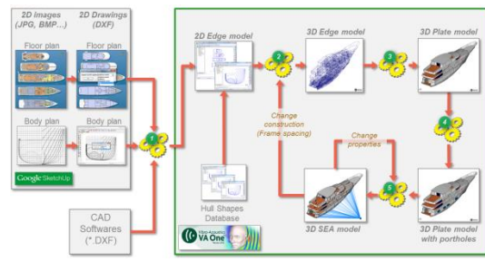
2D to 3D automatic SEA model building
