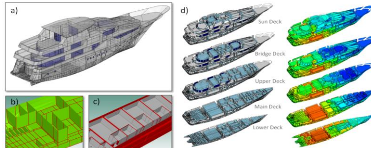
High frequency Acoustic Trim
