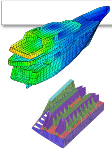
Low frequency Structural stiffness
