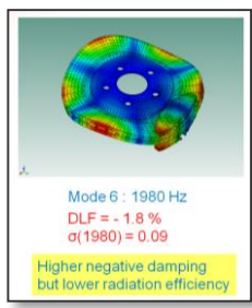
Break Squeal
