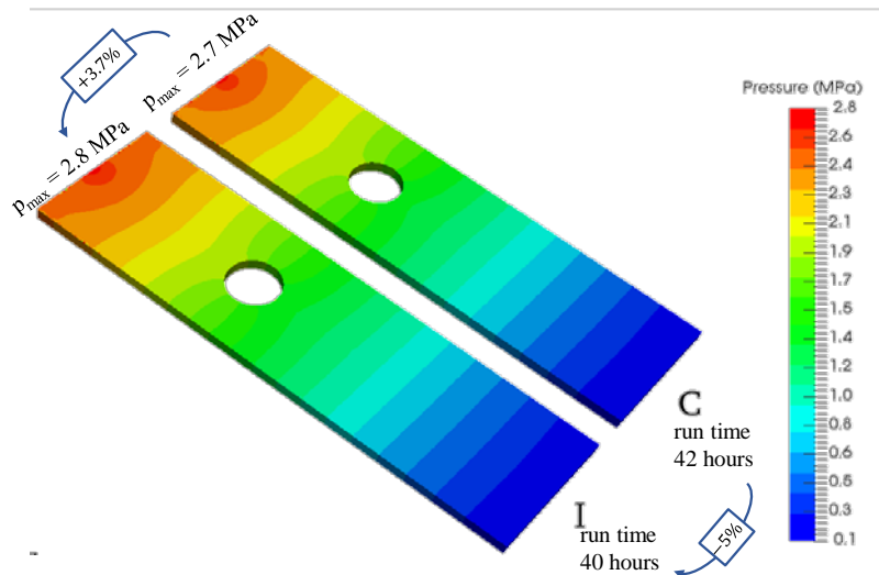
Figure 2. Distribution of the pressure field on the mold cavity, for the two formulations, compressible (C) and incompressible (I), at the switch-over point.
