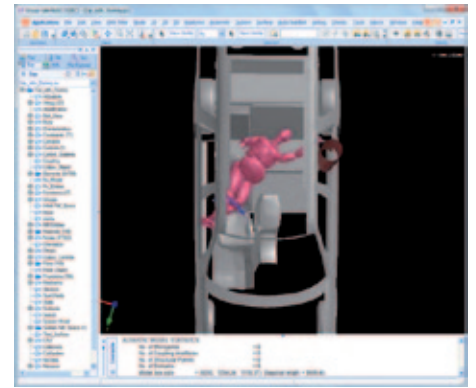
Maximum rearward excursion of belted occupant
