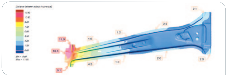
Figure 2: B-Pillar Inner: PAM-STAMP 2G results compared to physical testing, Isotropic Hardening Model. 52.3 % of the points within +/- 1mm
