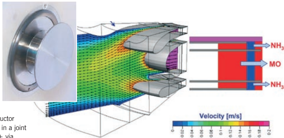
Figure 3: CFD modelling of a novel gas injector used in the AIXTRON Planetary Reactor®.
