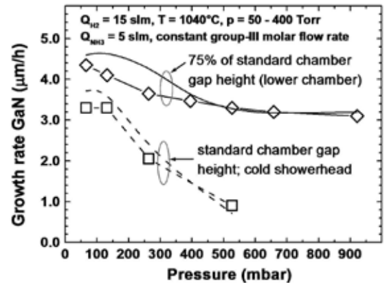
Figure 2: Pressure dependence of GaN growth rate in the 6x2" Close Coupled Showerhead Reactor, comparing two different hardware sets, (a) bare, cold showerhead and (b) covered warmer showerhead with reduced chamber height. Model prediction (lines without symbols) and experimental data (lines and symbols).
