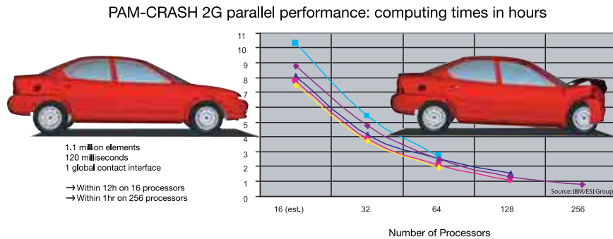
PAM-CRASH 2G parallel performance
